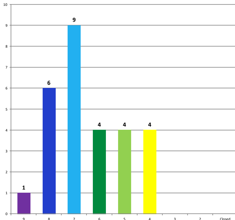
Number of Bridges by 2018 General Appraisal
