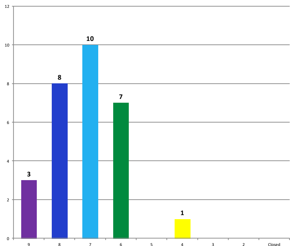
Number of Bridges by 2018 General Appraisal
