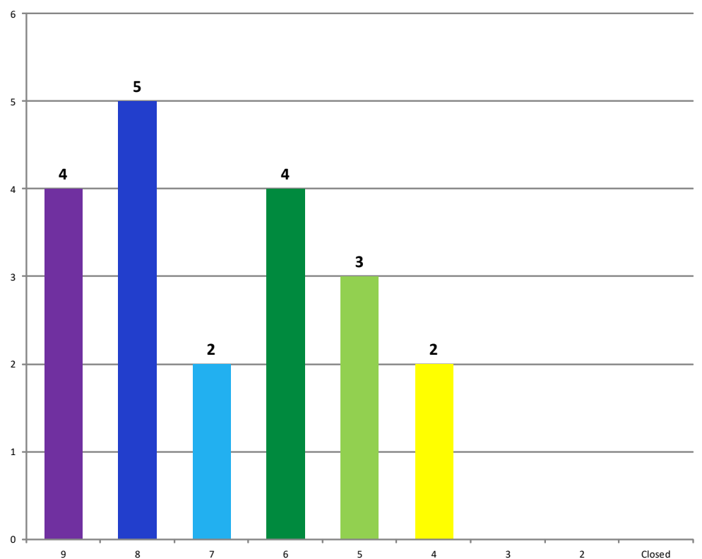
Number of Bridges by 2018 General Appraisal
