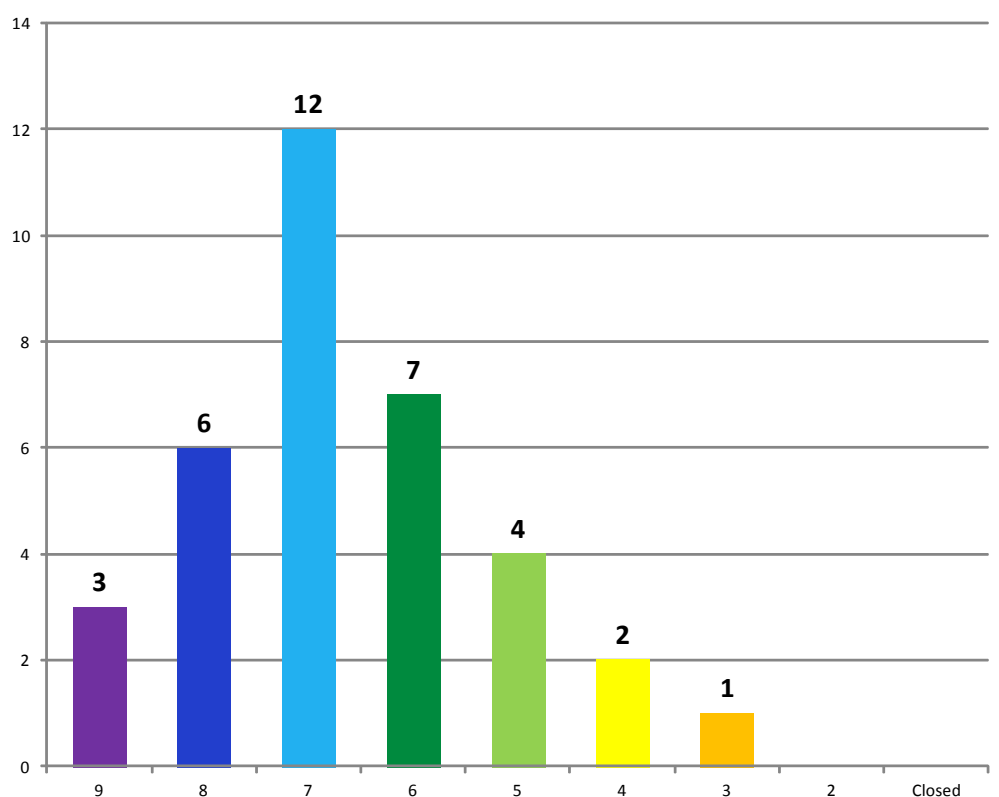
Number of Bridges by 2017 General Appraisal
