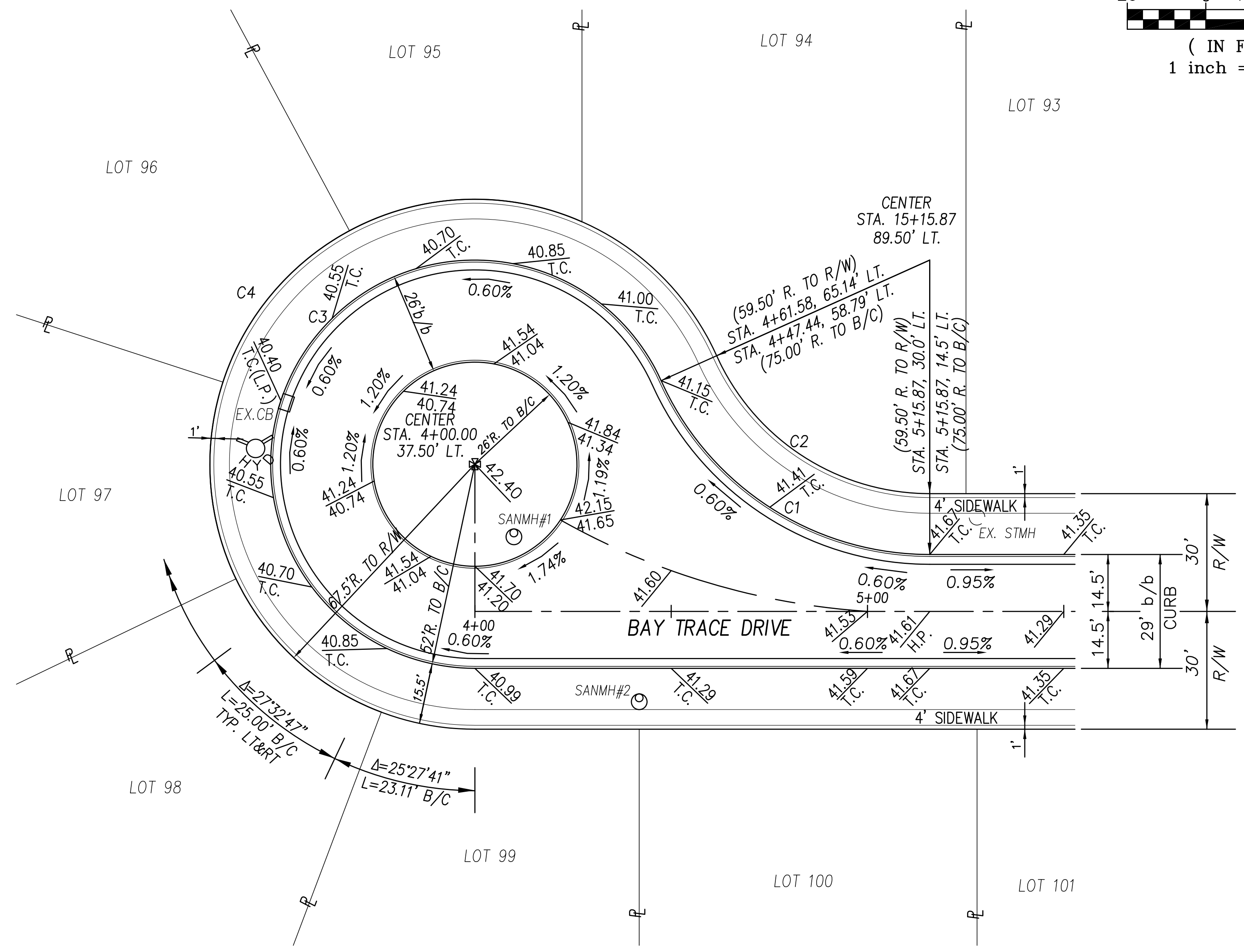
BAY TRACE DRIVE CUL-DE-SAC DETAIL (PLAT 5)
