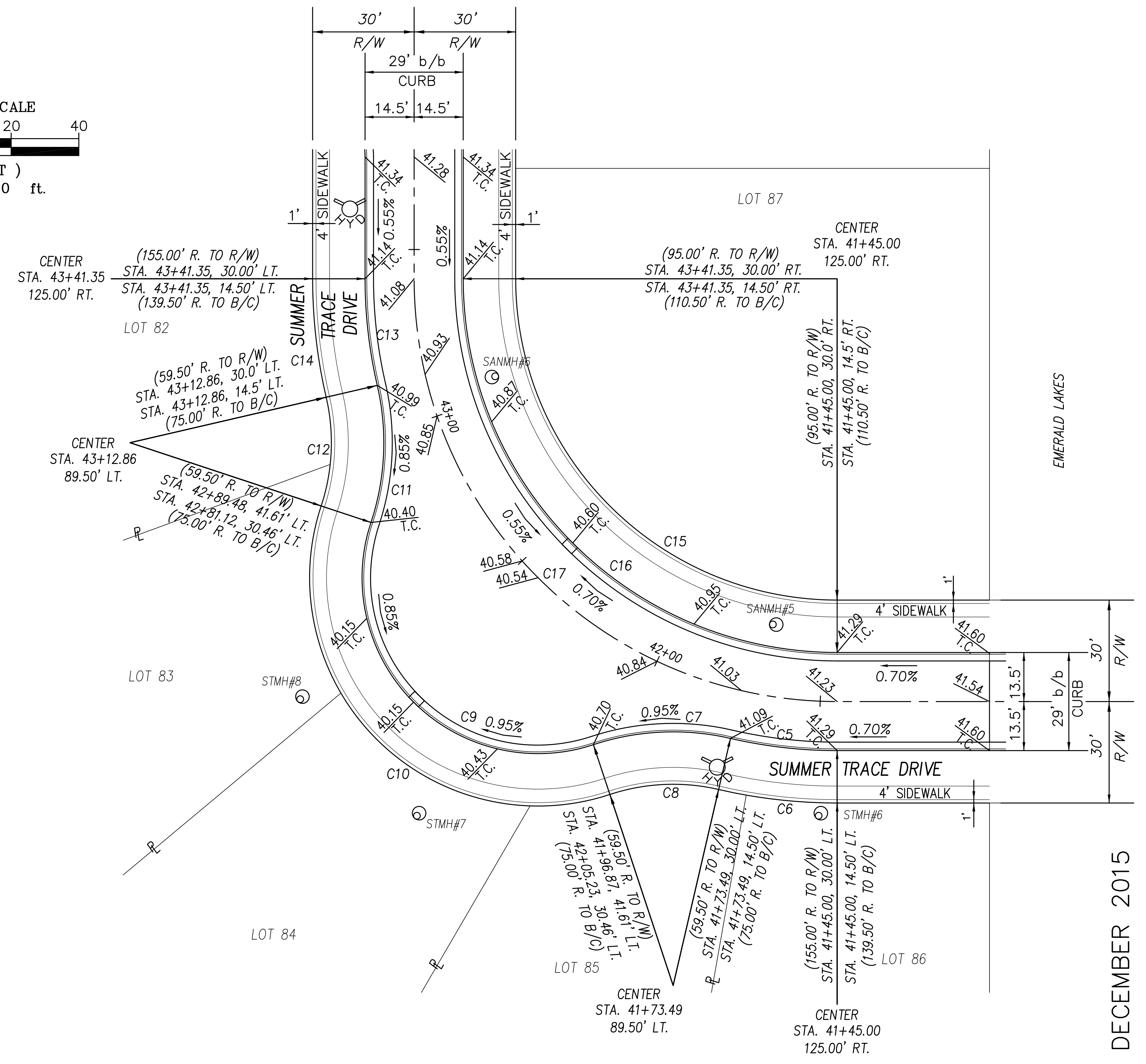
SUMMER TRACE DRIVE EYEBROW DETAIL (PLAT 4)
